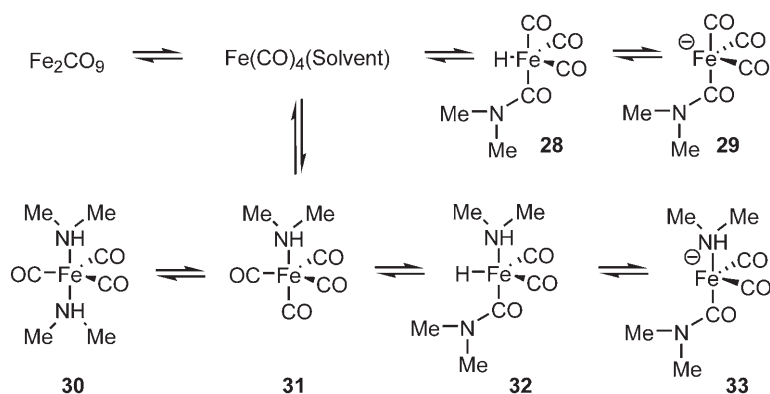
Scheme 1. Postulated structures of the nucleophiles generated from \text{Fe}_2(\text{CO})_9 and dimethylamine.
